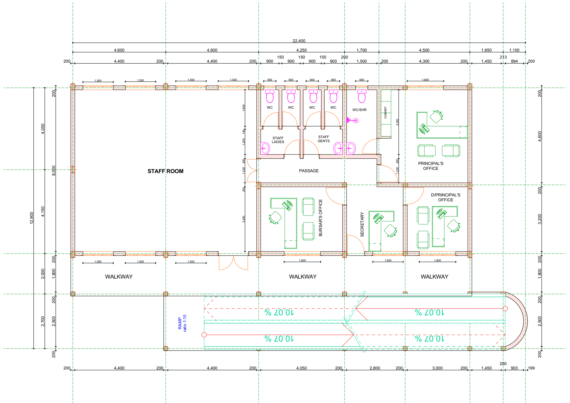
GROUND FLOOR LAYOUT PLAN
